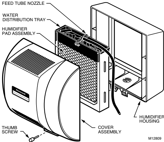
Fig. 13. Cleaning your humidifier.
