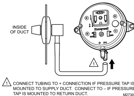
Fig. 10. Install tubing.
