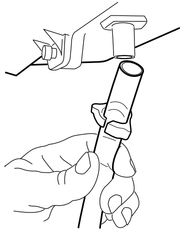
Fig. 7. Installing feed tubing.
