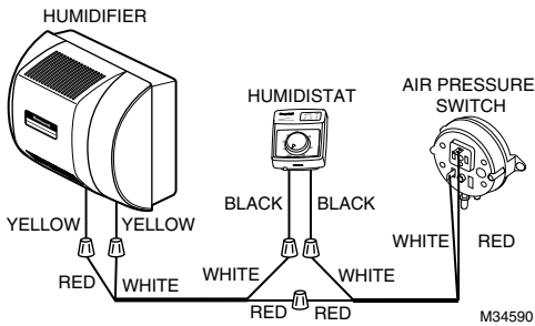
Fig. 12. Wiring the controls.
