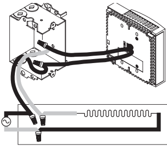
2-wire Installation
